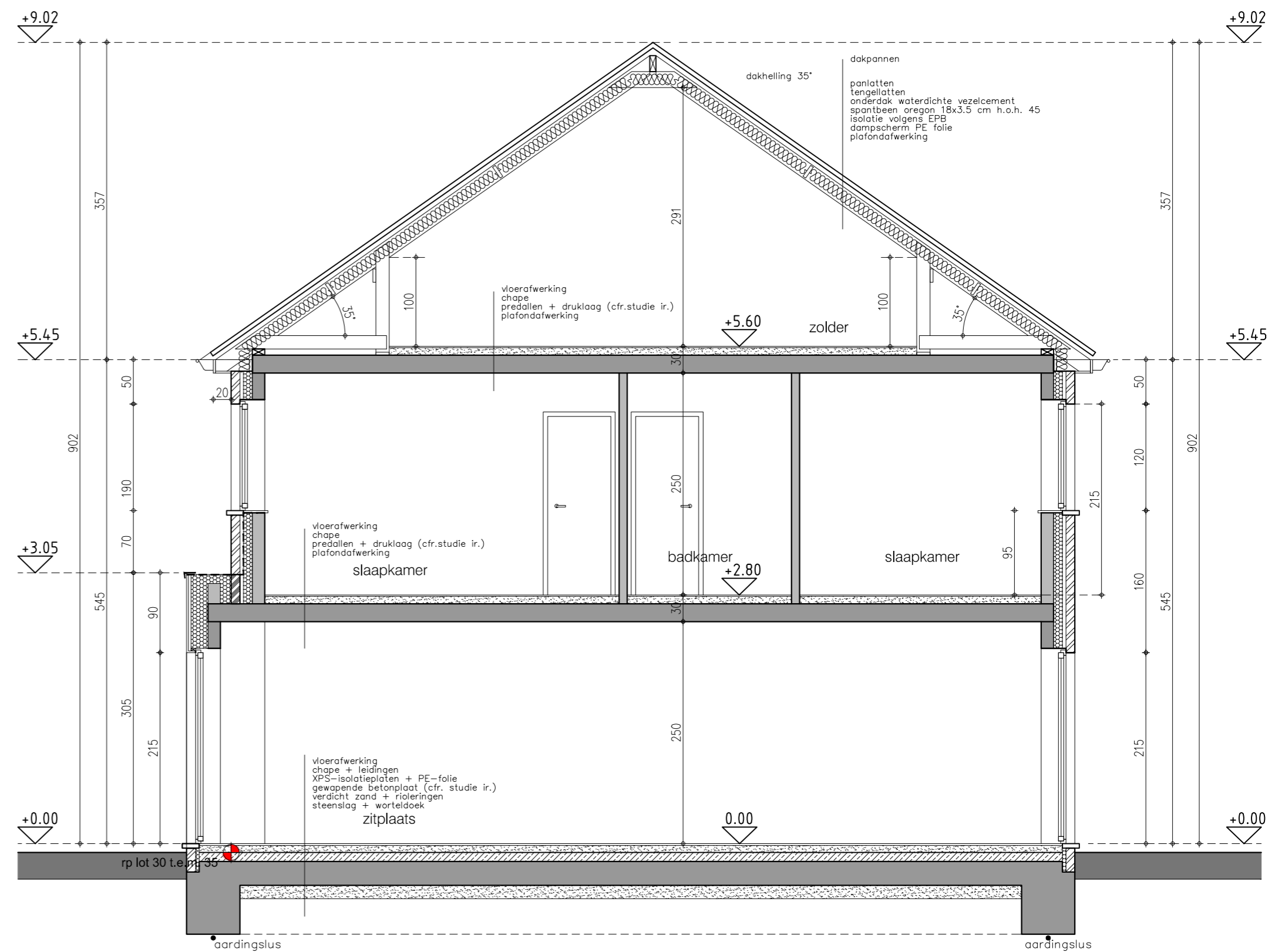
doorsnede C2 - C2 lot 31 - 33 typesnede lot 30 - 35
